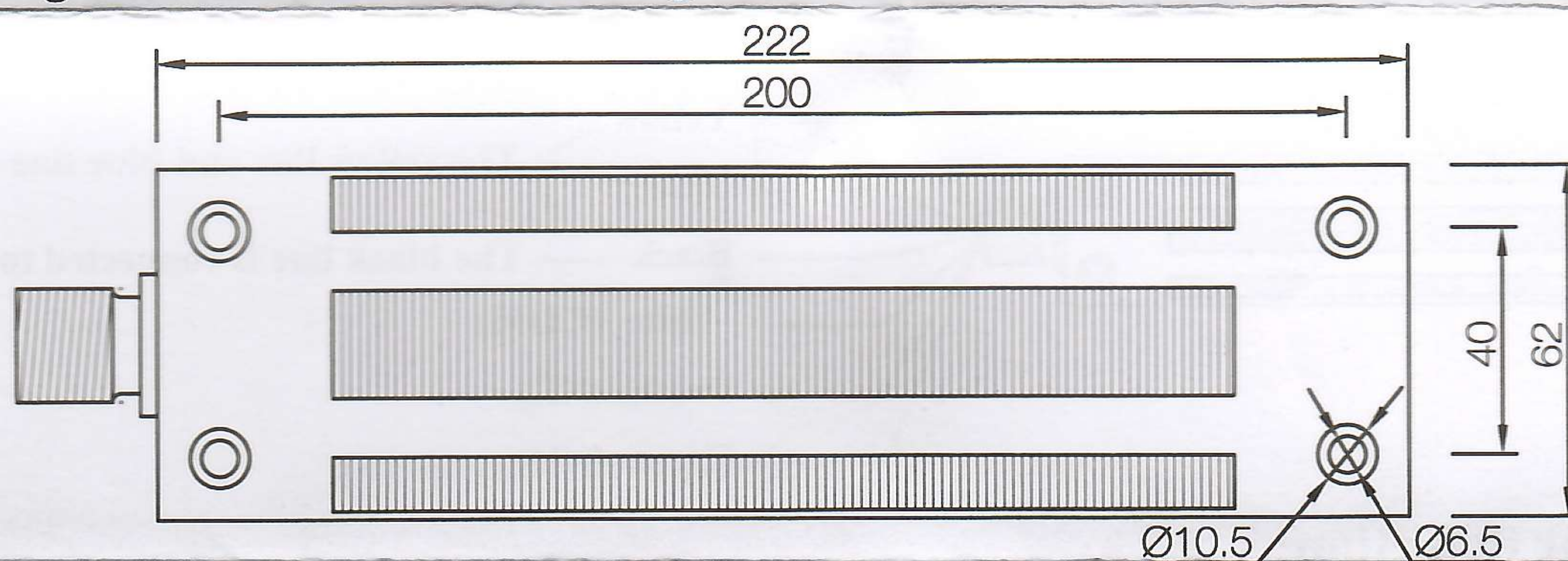
Magnetic lock dimension drawing
